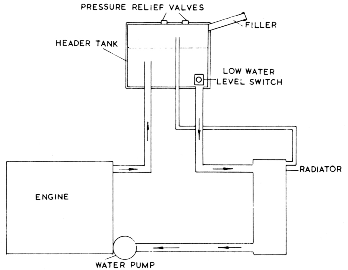
PRESSURISED SYSTEM
