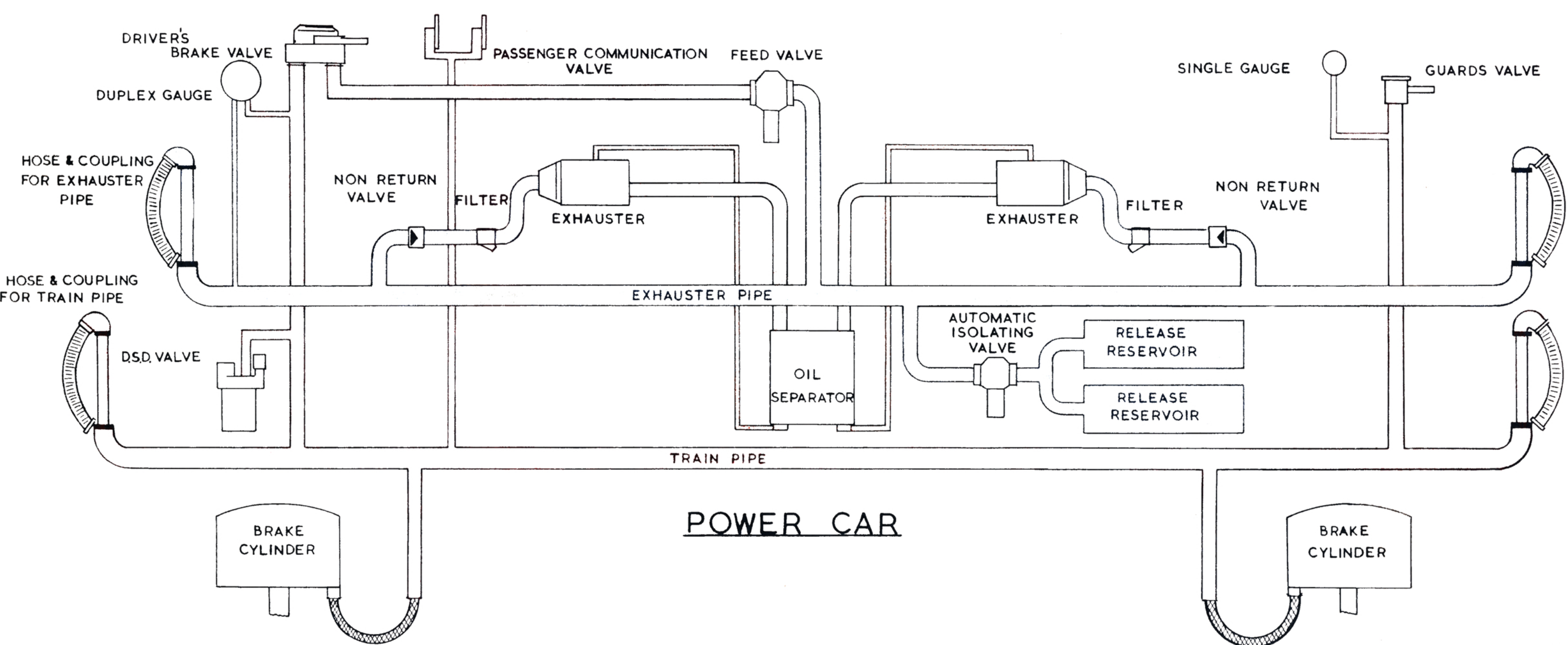
QUICK RELEASE VACUUM BRAKE SYSTEM
