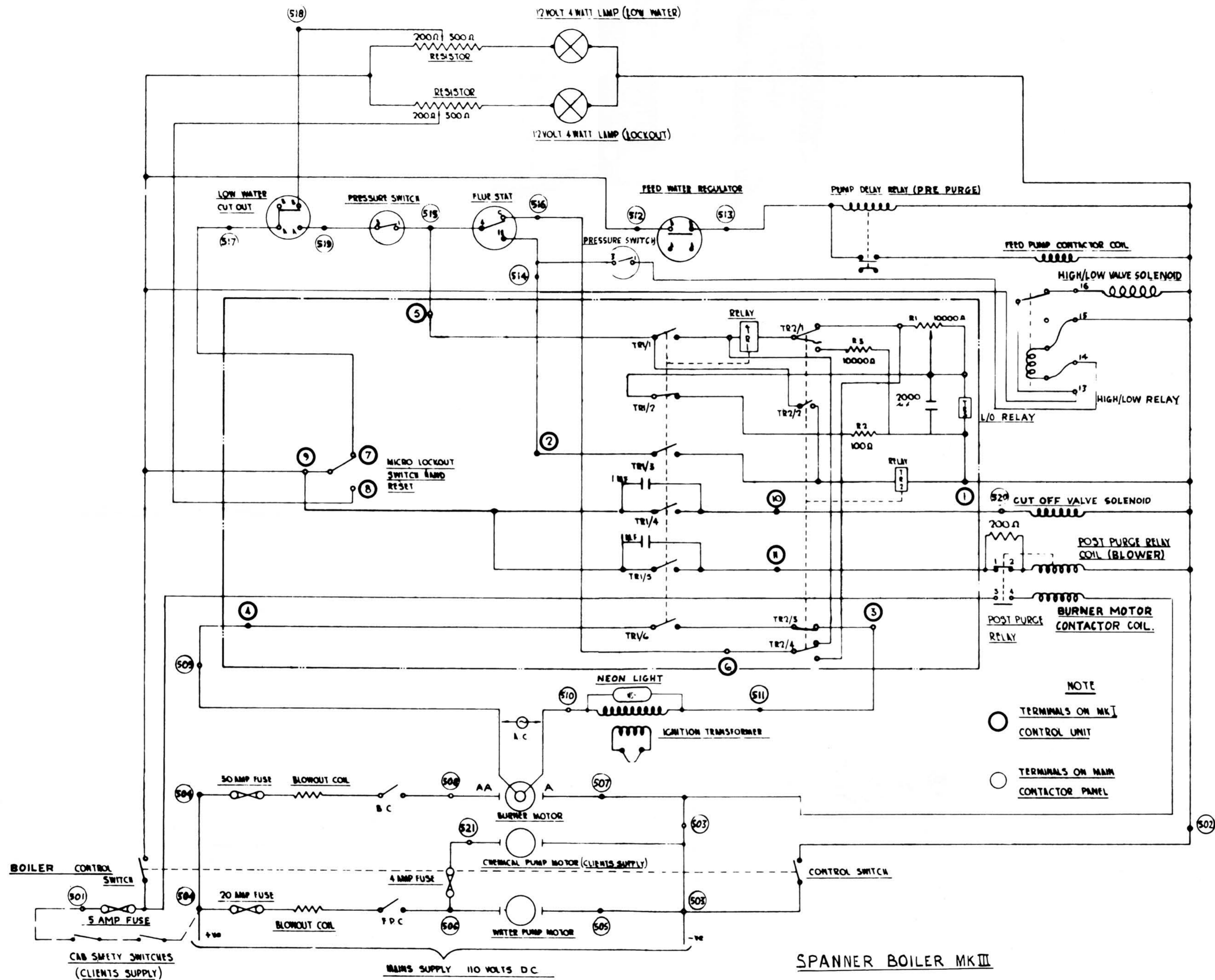
LINE WIRING DIAGRAM FOR TRAIN HEATING BOILER. (TYPICAL)
